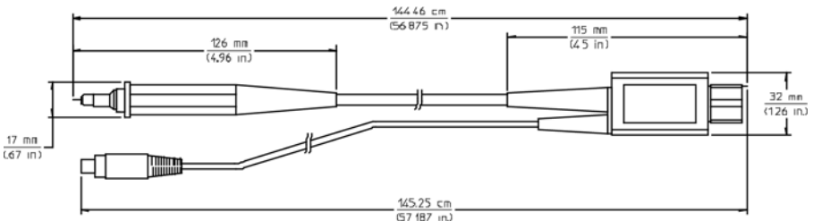
1144A Dimensions.
