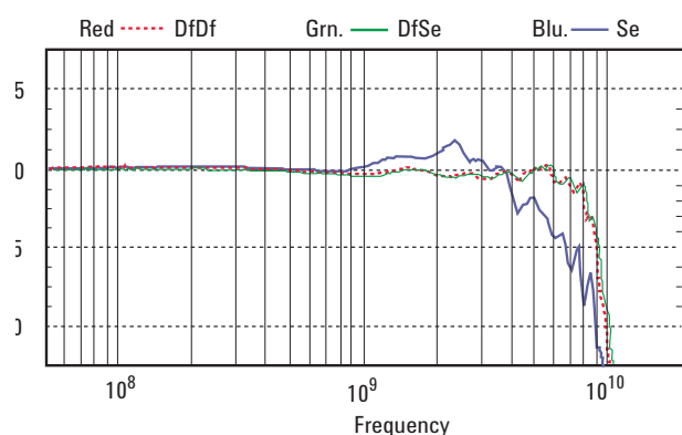
Figure 4. Frequency response of differential and single-ended probes
