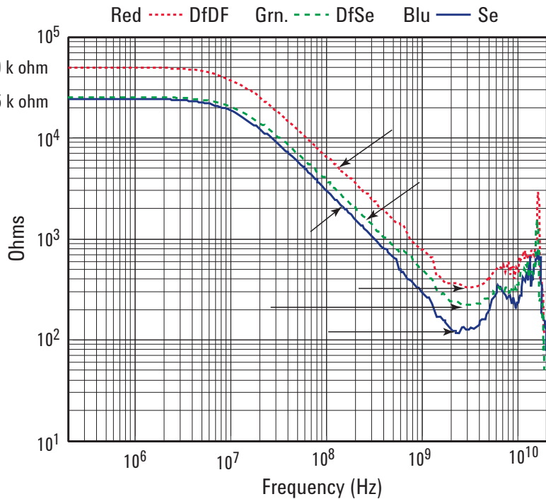
Figure 8. Input impedance of differential and single-ended probes
