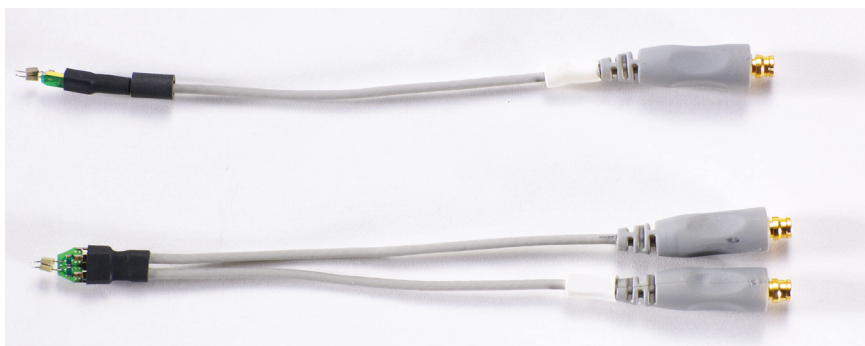
Figure 2. Keysight 1134A single-ended solder-in probe head (top), and differential solder-in probe head (bottom)
