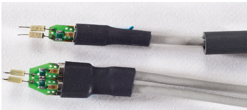
Figure 3. Close up of single-ended (top) and differential (bottom) solder-in probe heads
