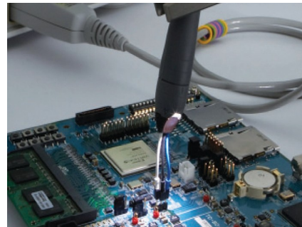
N2750A-02A InfiniiMode probe with standard accessories
