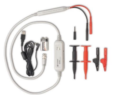
N2792A 200-MHz, 20-V differential probe with standard accessories
