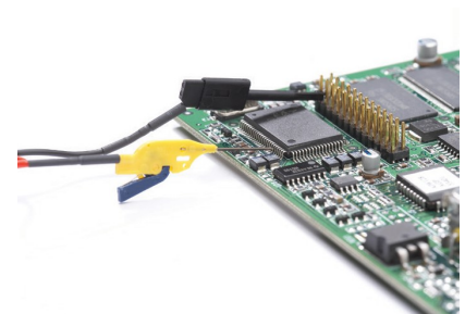
IC clips included in N2877A and N2878A accessory kits for N2870A Series passive probes
