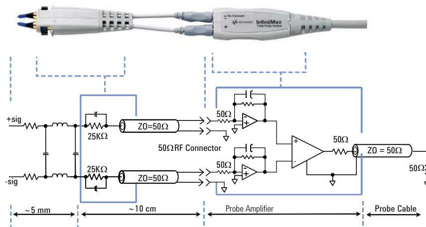
Figure 1. InfiniiMax architecture
