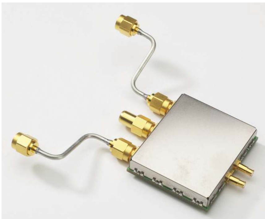
Figure 8. N5380A dual-SMA differential probe head
