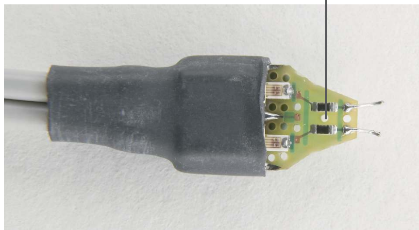
Figure 2. InfiniiMax solder-in probe head detail
