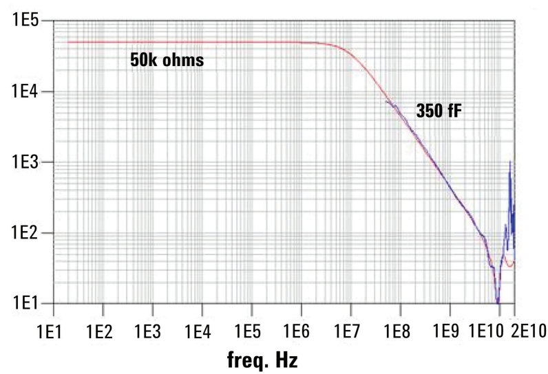
Figure 3 Differential Input Impedance plot, input C = ~0.72 pF
