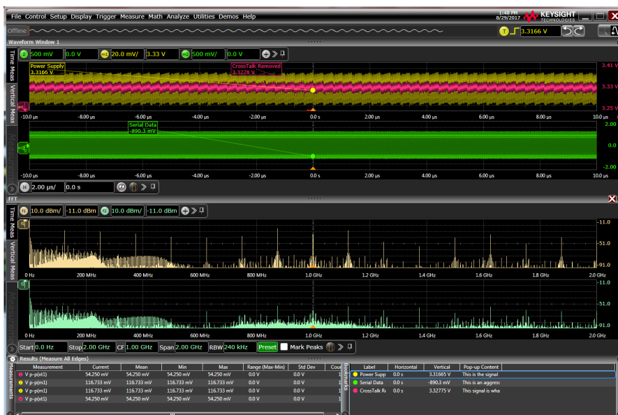
Figure 30. Output from the N8846A PI application showing a reduction in the noise on the 3.3 V supply after the affects of the switching loads were removed.
