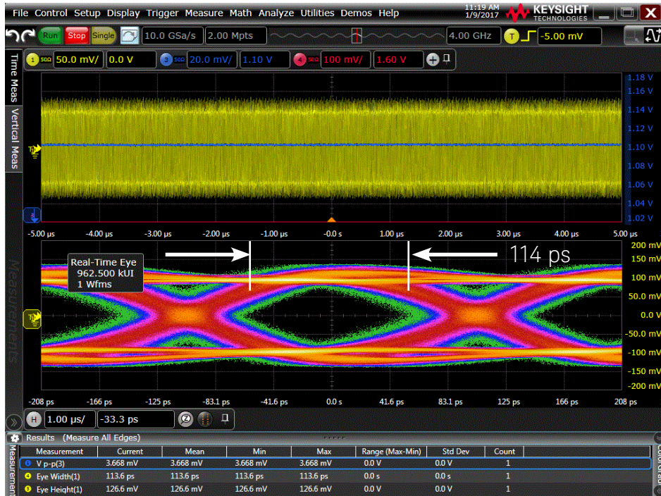
Figure 25. Eye diagram of FPGA serial data after the DC supply was cleaned-up. Notice the increased width of the eye.
