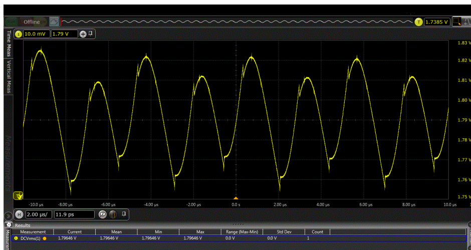
Figure 1. Using the N7020A power rail probe, with 2 GHz bandwidth and 50 k \Omega DC resistive loading, to see the AC and DC components of a DC power rail.
