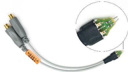
Figure 9: N5381B differential solder-in head
