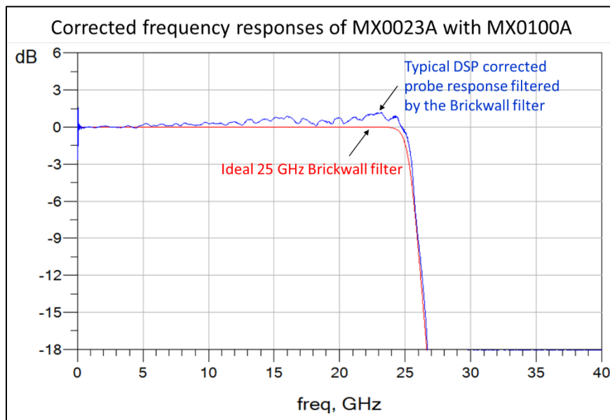
Figure 3: The unique s parameter of the probe amp is used to flatten the magnitude and phase response of the probe for high accuracy measurements.
