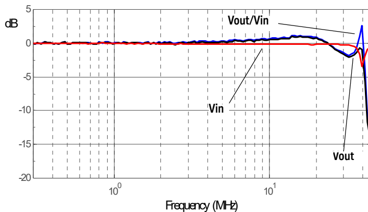
Figure 4 Graph of dB(V_{in}) , dB(V_{out}) + 20dB , and dB(V_{out}/V_{in}) + 20dB frequency response, 10:1 attenuation
