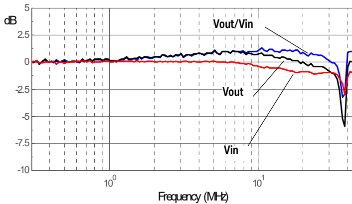
Figure 5 Graph of dB(V_{in}) , dB(V_{out}) + 40dB , and dB(V_{out}/V_{in}) + 40dB frequency response, 100:1 attenuation
