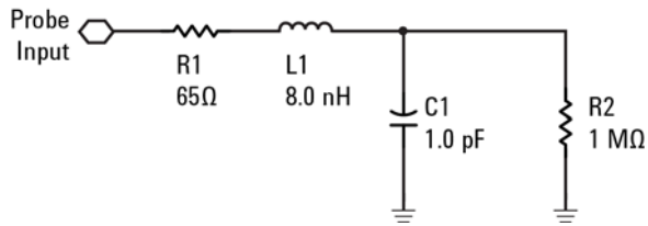
Figure 14 Input Impedance Equivalent Model
