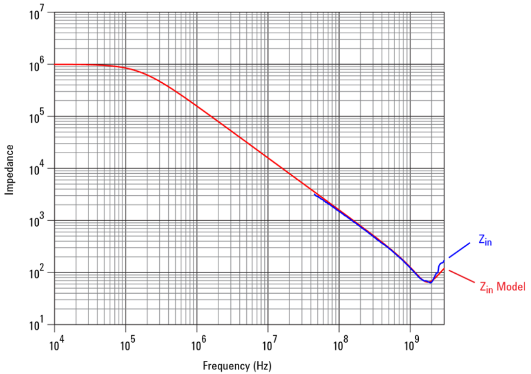
Figure 15 Typical Input Impedance Plot
