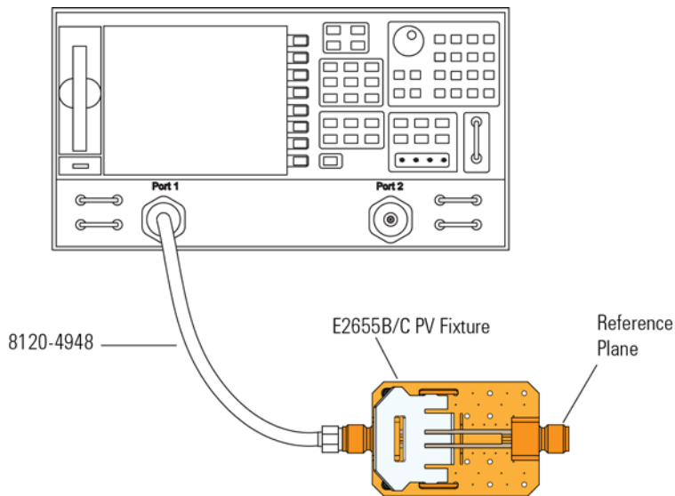
Figure 17 PV Fixture Connected to VNA
