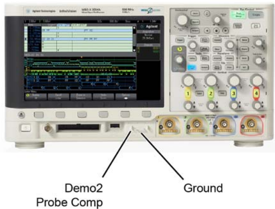
Figure 12 Probe Calibration Terminals on 3000 X-Series Oscilloscope
