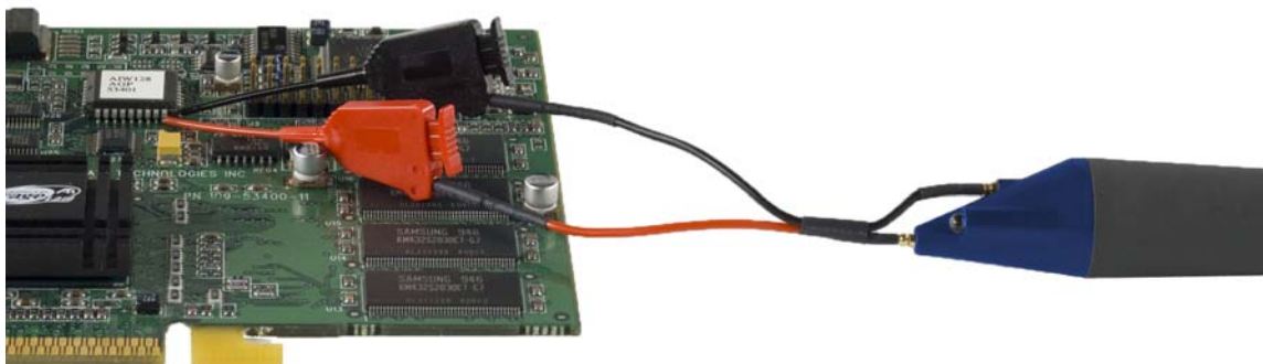
Figure 9 Probe with Flexible Nose Clips Attached
