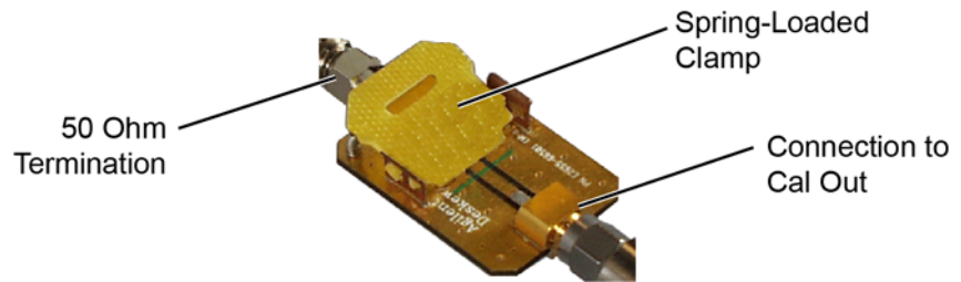
Figure 11 E2655B PV Fixture with 50 Ohm Termination
