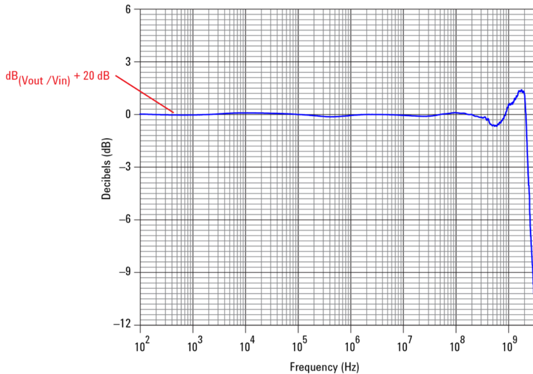
Figure 13 Frequency Response (Vout/Vin)
