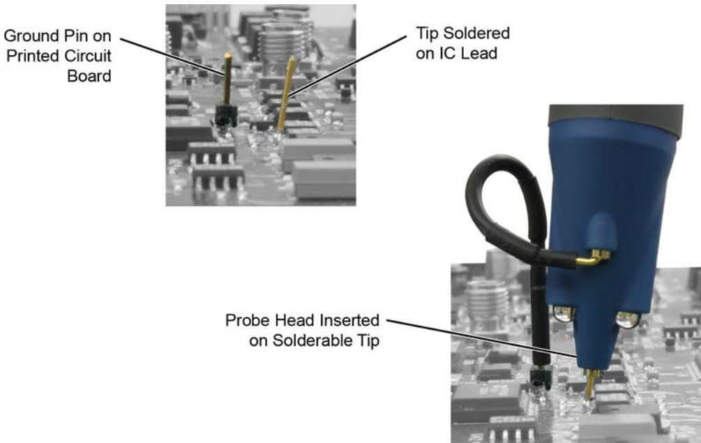
Figure 6 Placing the Probe Onto the Solderable Tip
