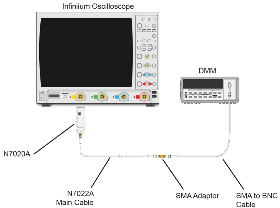
Figure 27 Test Setup
