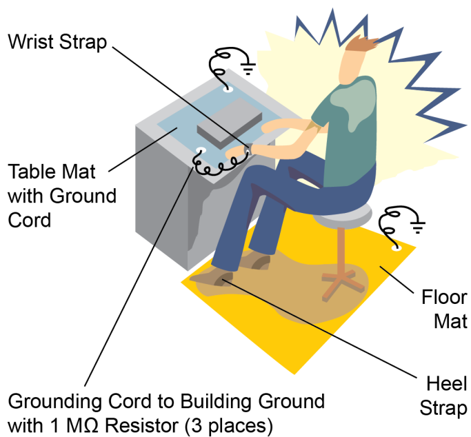
Figure 11 ESD Workstation
